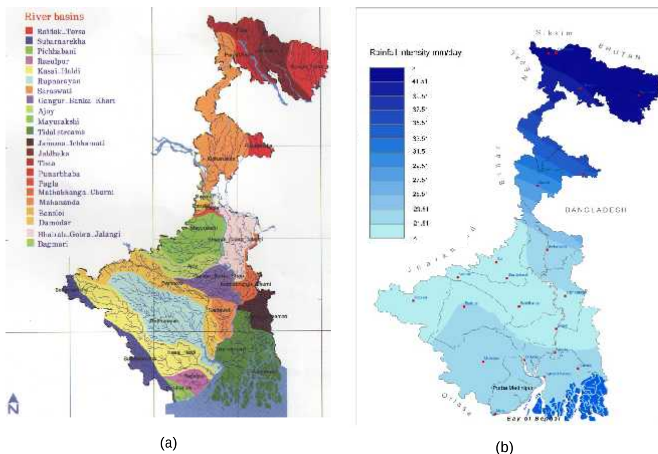
Figure 5.1: (a) Drainage basins of West Bengal, (b) Rainfall intensity across West Bengal
