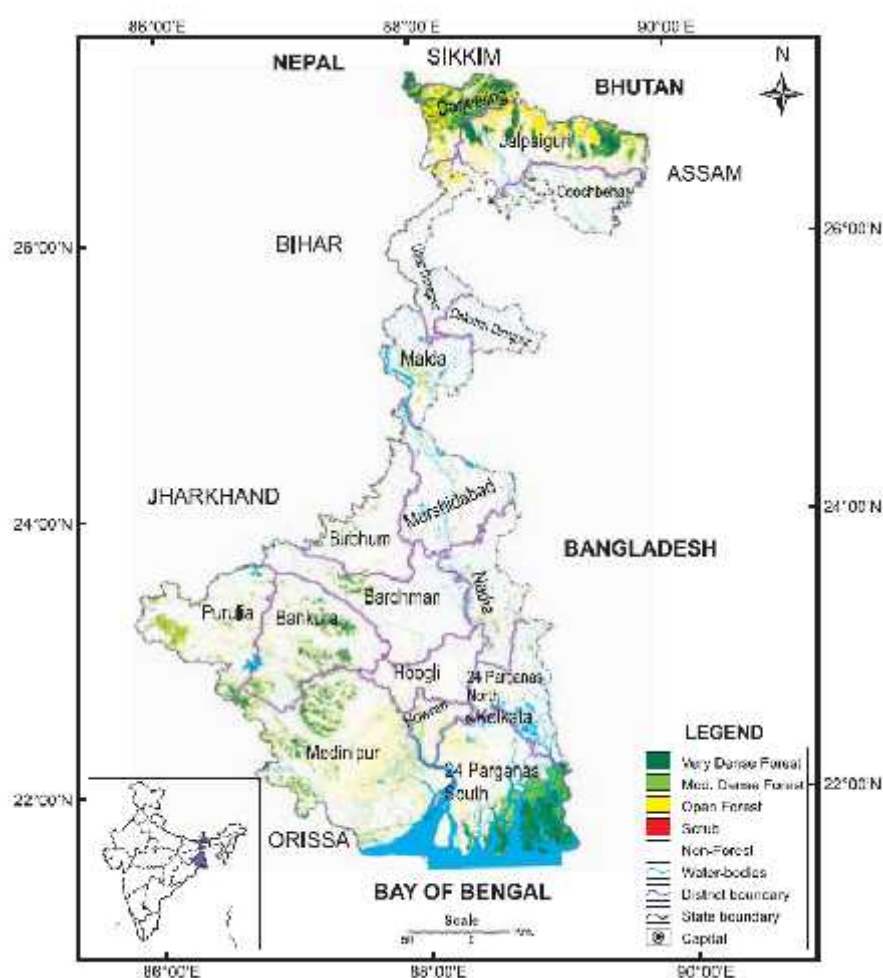
Figure 7.1: Forest Cover Map of West Bengal.
